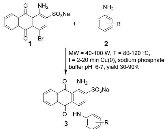
Scheme 2. Microwave-Assisted Cu(0)-Catalyzed Synthesis of Anilinoanthraquinone Derivatives in Phosphate Buffer
