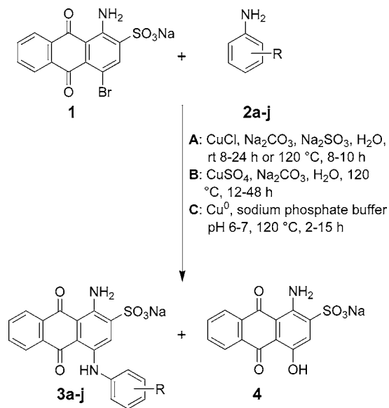
Scheme 1. Syntheses of Anilinoanthraquinone Derivatives
